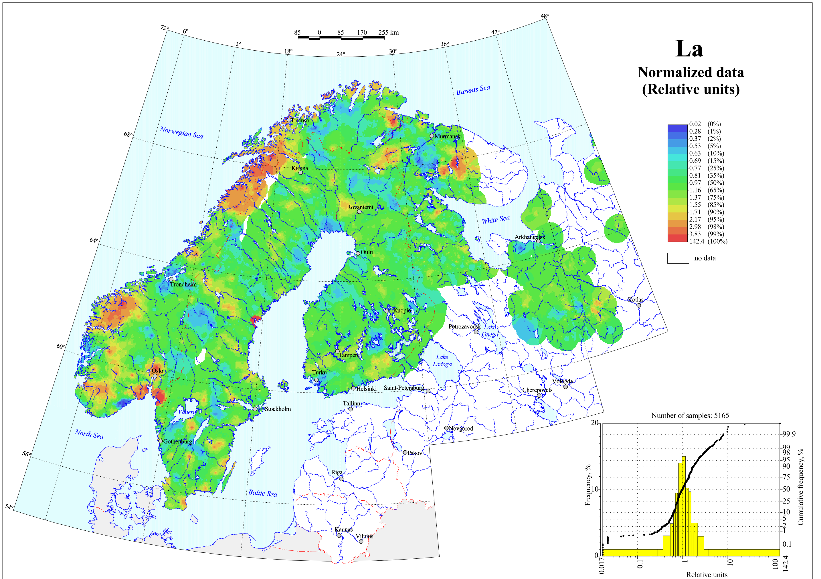
Lanthanum in Till, Grain Size <0.06 mm
